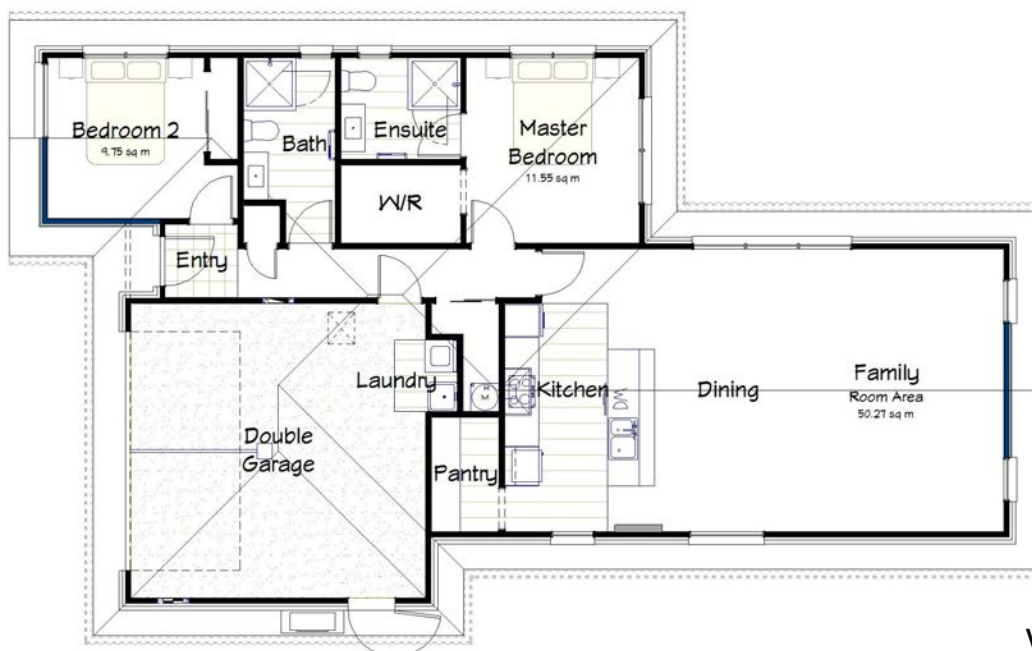
Floor Plan
